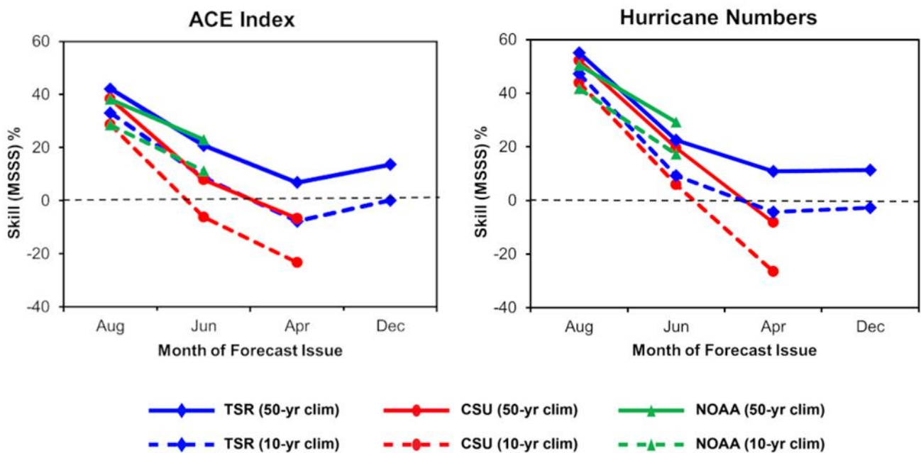
Figure 3. Real-time skill of North Atlantic seasonal tropical cyclone outlooks assessed for the 19-year period 2003-2022. The skill of the seasonal outlooks issued publicly by Tropical Storm Risk (TSR, blue lines), Colorado State University (CSU, red lines), and the National Oceanic and Atmospheric Administration (NOAA, green lines) are compared for ACE (left panel) and for hurricane numbers (right panel). The skill is shown as the Mean Square Skill Score (MSSS) based on a fixed 50-year (1951-2000) climatology and on a running prior 10-year climate norm.
